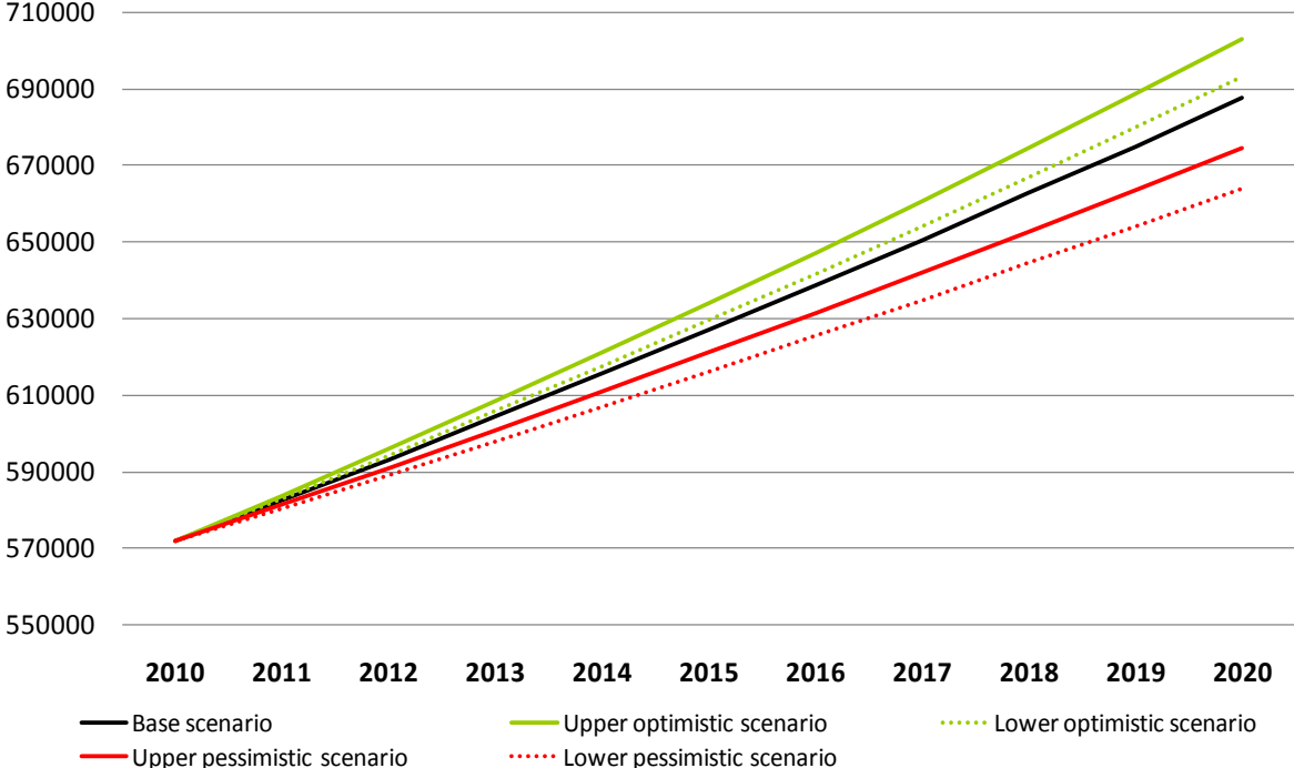
Implications of base, optimistic, and pessimistic scenarios for future GDP, million EUR, constant 2006 prices
